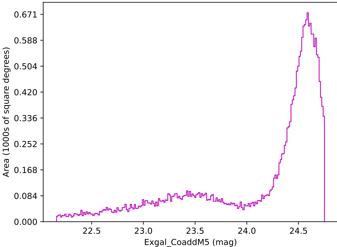
weather_cloudso2v3.4_10yrs Yr 1 z band: Exgal_CoaddM5
