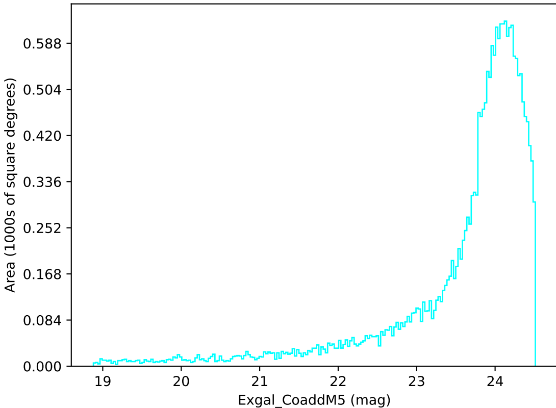
weather_cloudso2v3.4_10yrs Yr 1 u band: Exgal_CoaddM5
