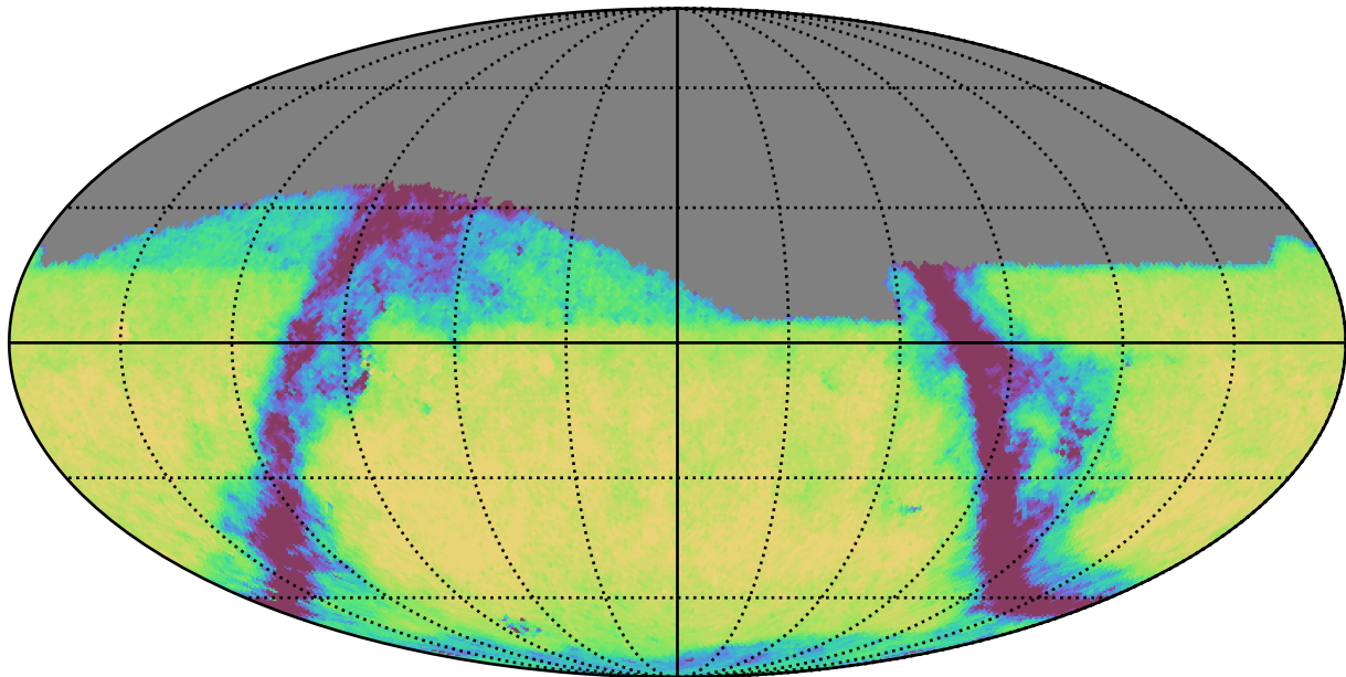
weather_cloudso2v3.4_10yrs Yr 1 r band: Exgal_CoaddM5
