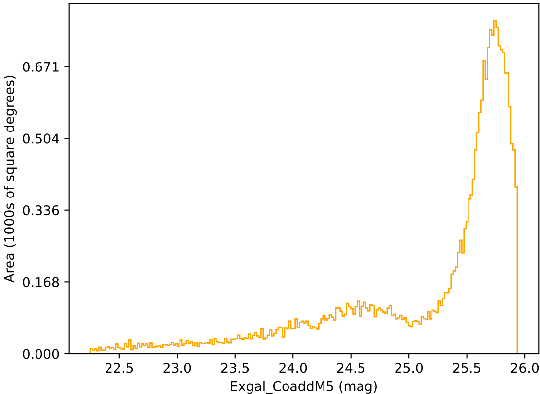
weather_cloudso2v3.4_10yrs Yr 1 r band: Exgal_CoaddM5
