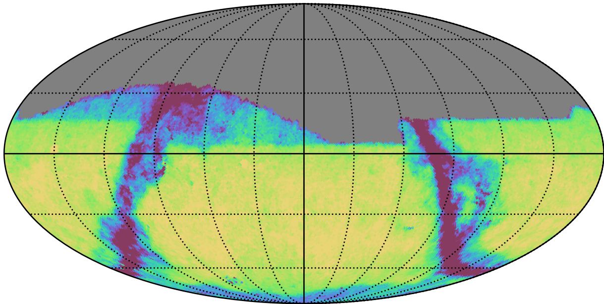
weather_cloudso2v3.4_10yrs Yr 1 i band: Exgal_CoaddM5
