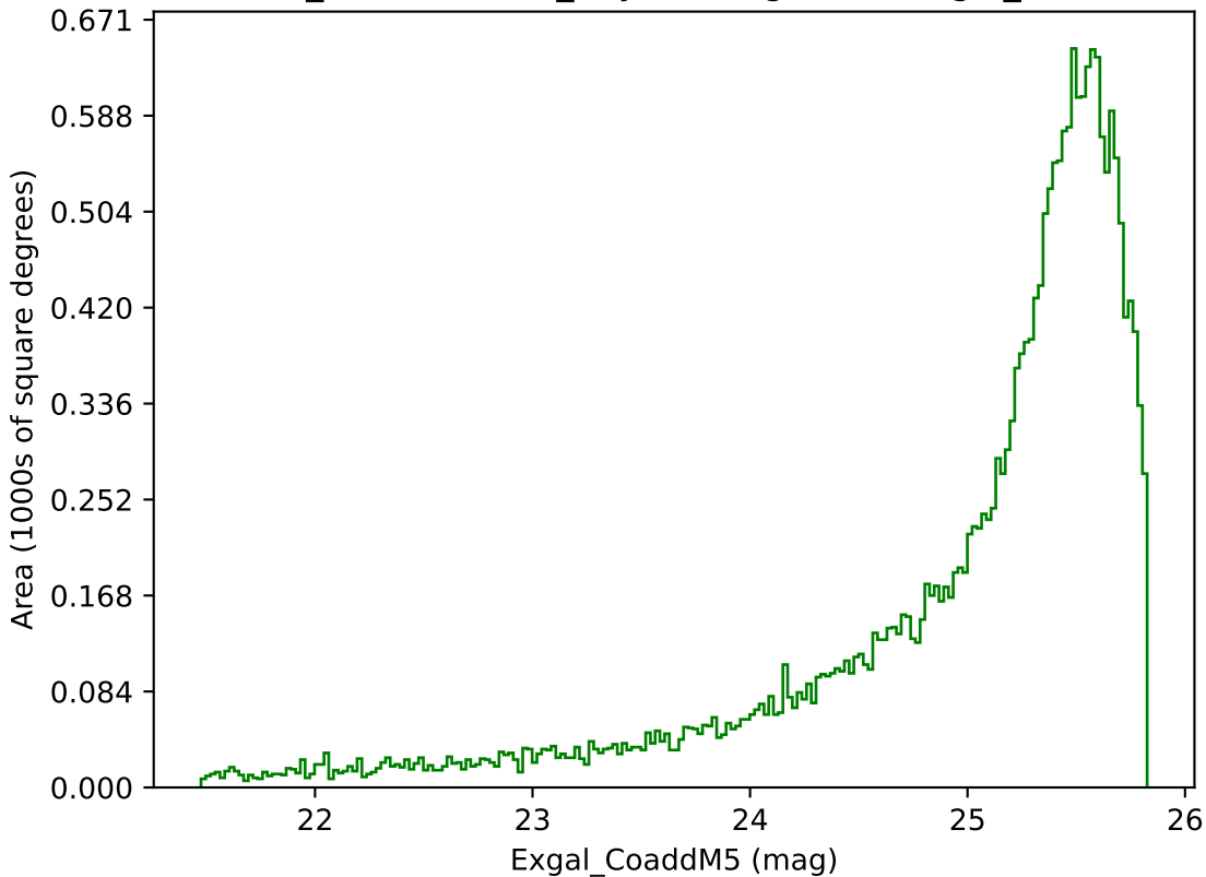
weather_cloudso2v3.4_10yrs Yr 1 g band: Exgal_CoaddM5
