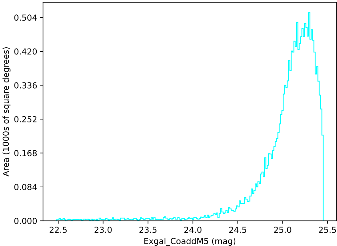
weather_cloudso2v3.4_10yrs WFD u band: Exgal_CoaddM5
