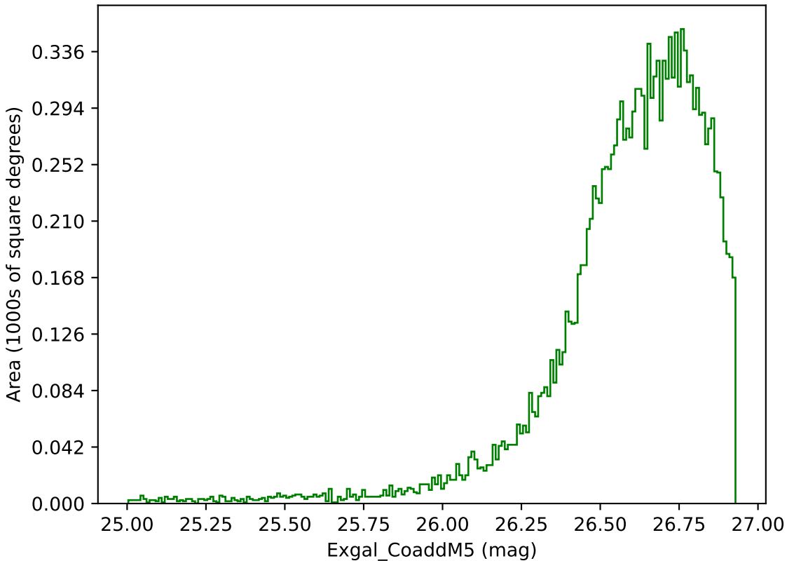
weather_cloudso2v3.4_10yrs WFD g band: Exgal_CoaddM5
