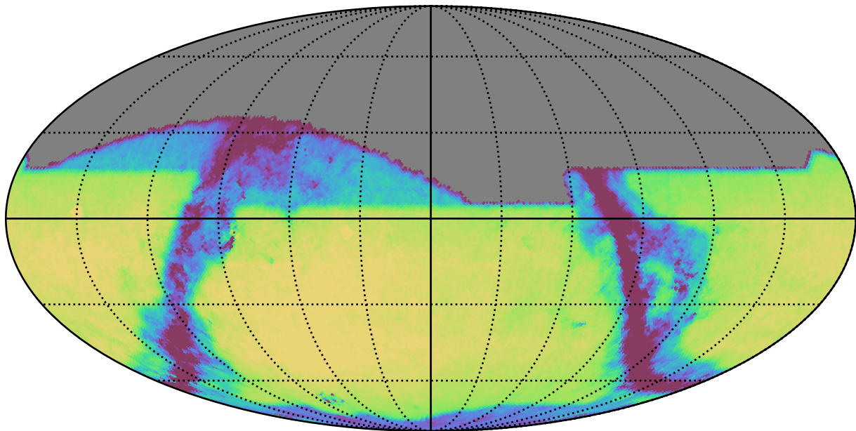
weather_cloudso2v3.4_10yrs All sky z band: Exgal_CoaddM5
