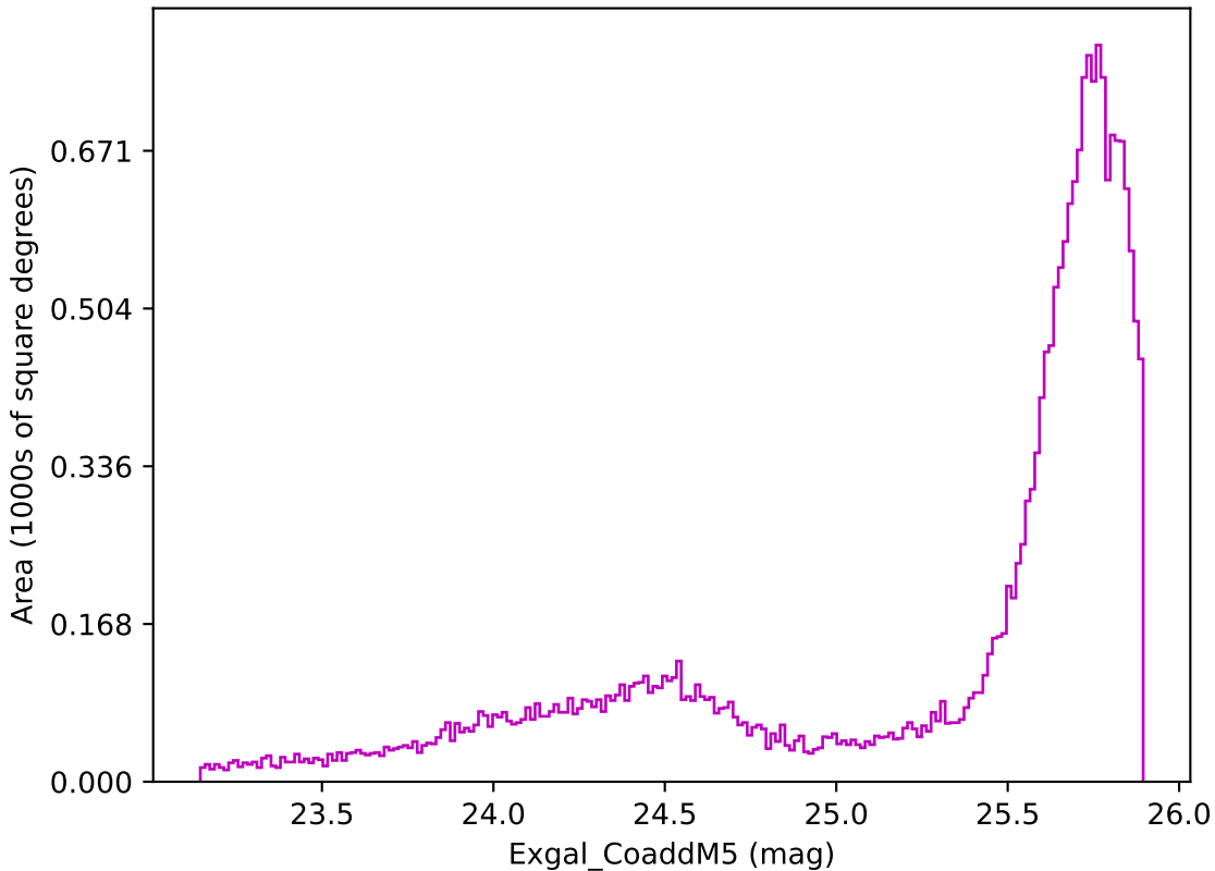
weather_cloudso2v3.4_10yrs All sky z band: Exgal_CoaddM5
