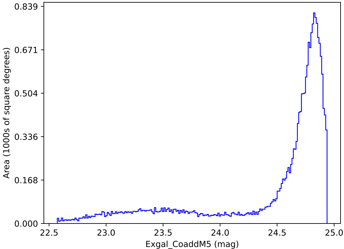
weather_cloudso2v3.4_10yrs All sky y band: Exgal_CoaddM5
