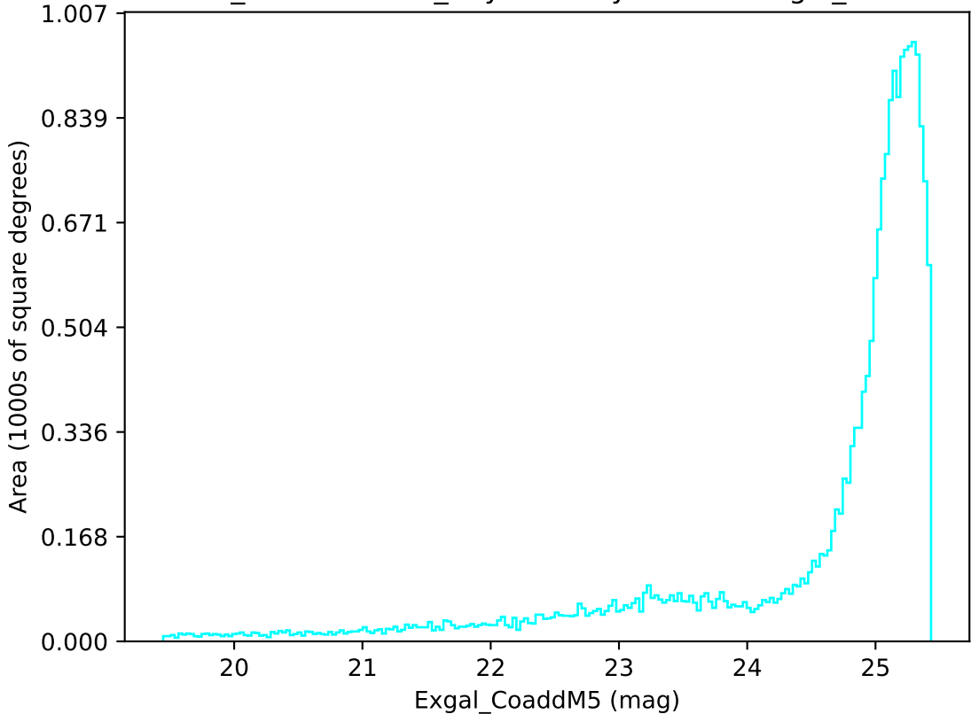
weather_cloudso2v3.4_10yrs All sky u band: Exgal_CoaddM5
