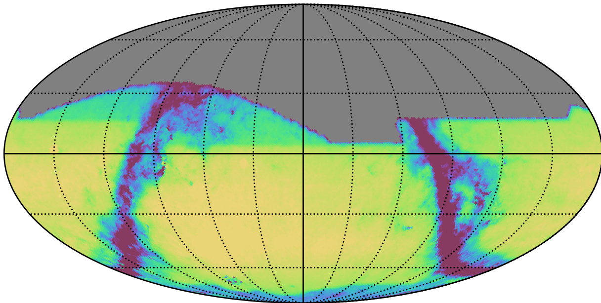
weather_cloudso2v3.4_10yrs All sky r band: Exgal_CoaddM5
