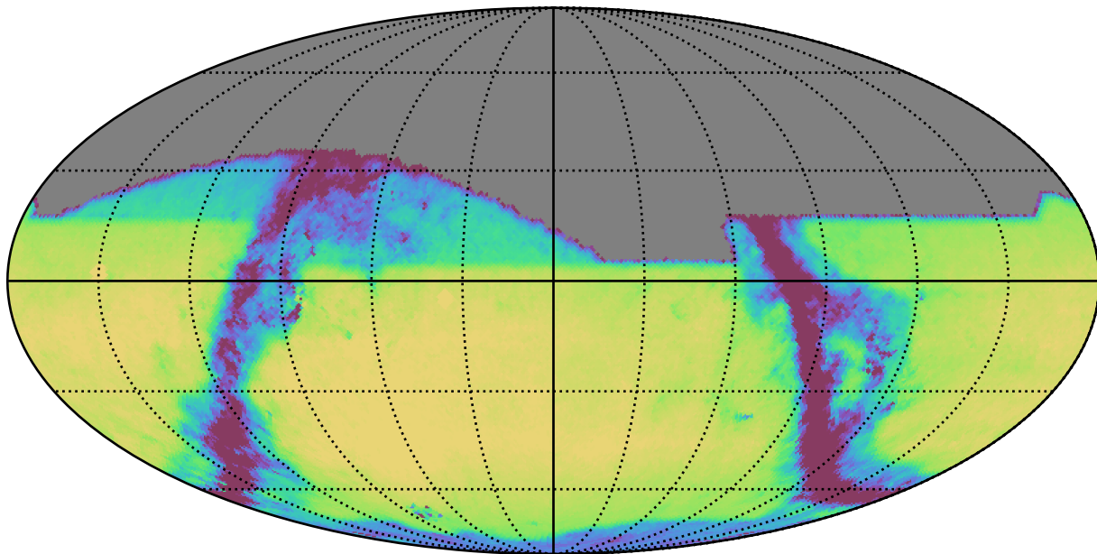
weather_cloudso2v3.4_10yrs All sky i band: Exgal_CoaddM5
