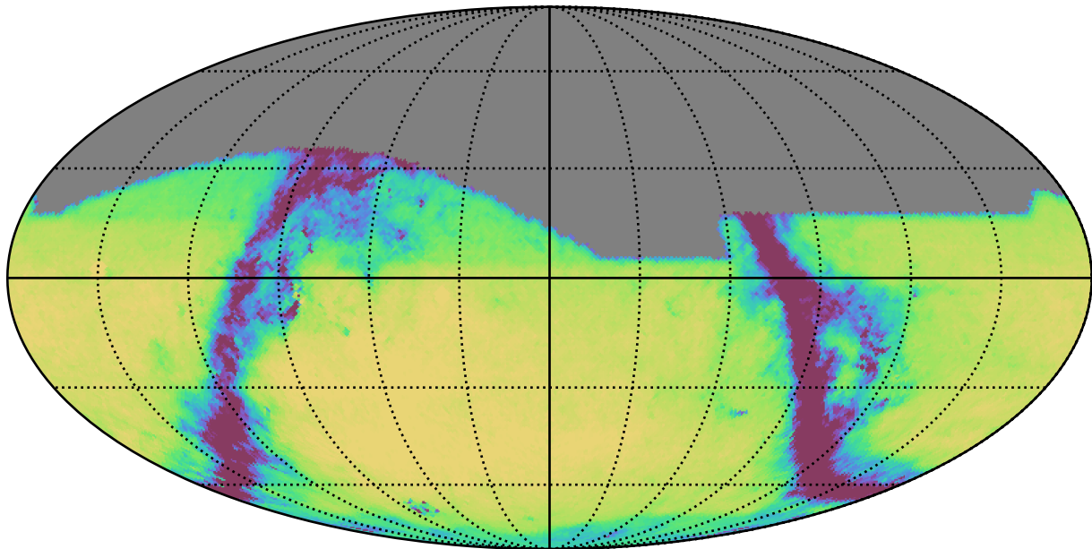
weather_cloudso2v3.4_10yrs All sky g band: Exgal_CoaddM5
