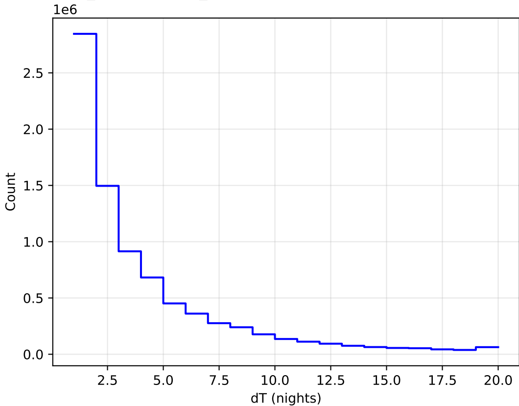
weather_cloudso2v3.4_10yrs WFD all bands: DeltaNight Histogram
