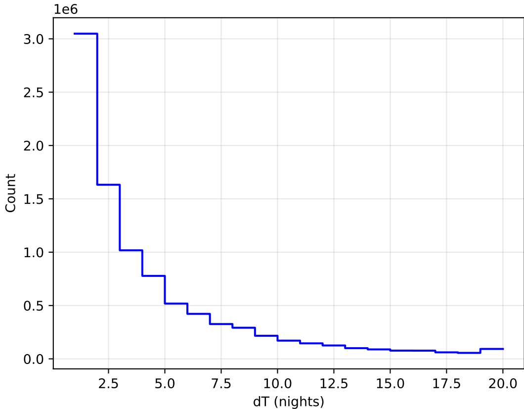
weather_cloudso2v3.4_10yrs All sky all bands: DeltaNight Histogram
