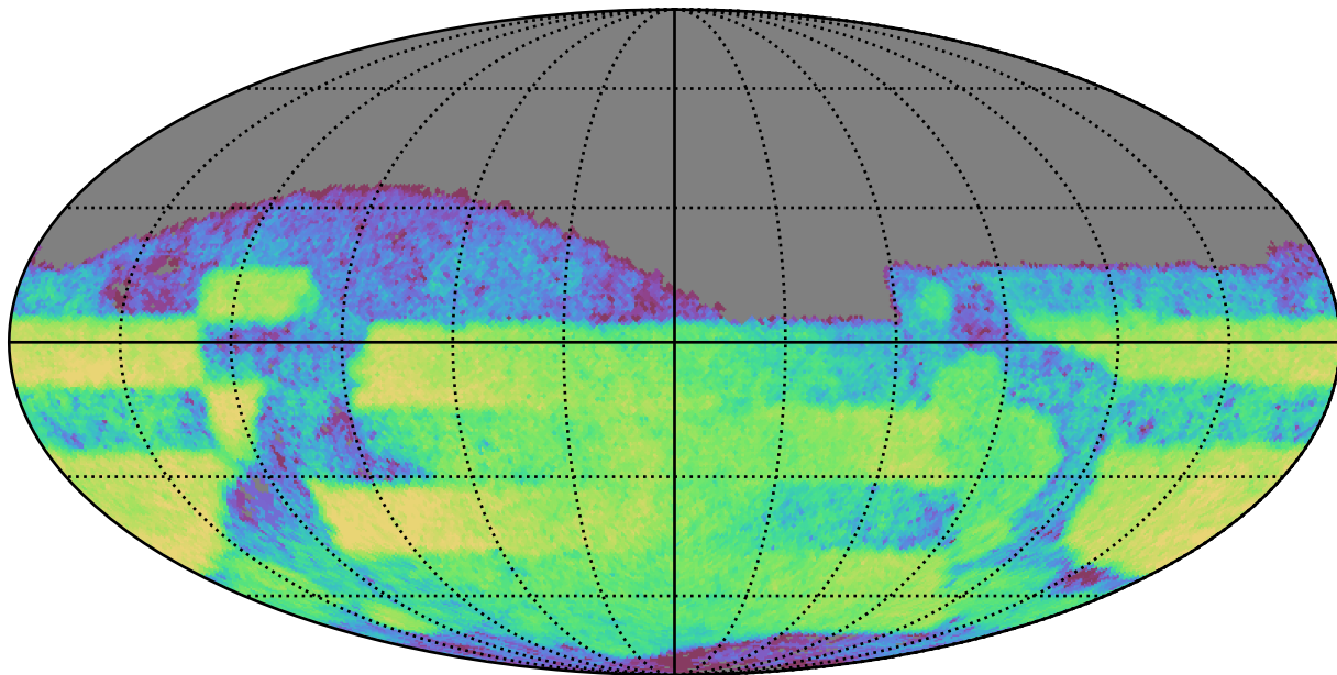
weather_cloudso2v3.4_10yrs Yr 3-4 z band: CoaddM5
