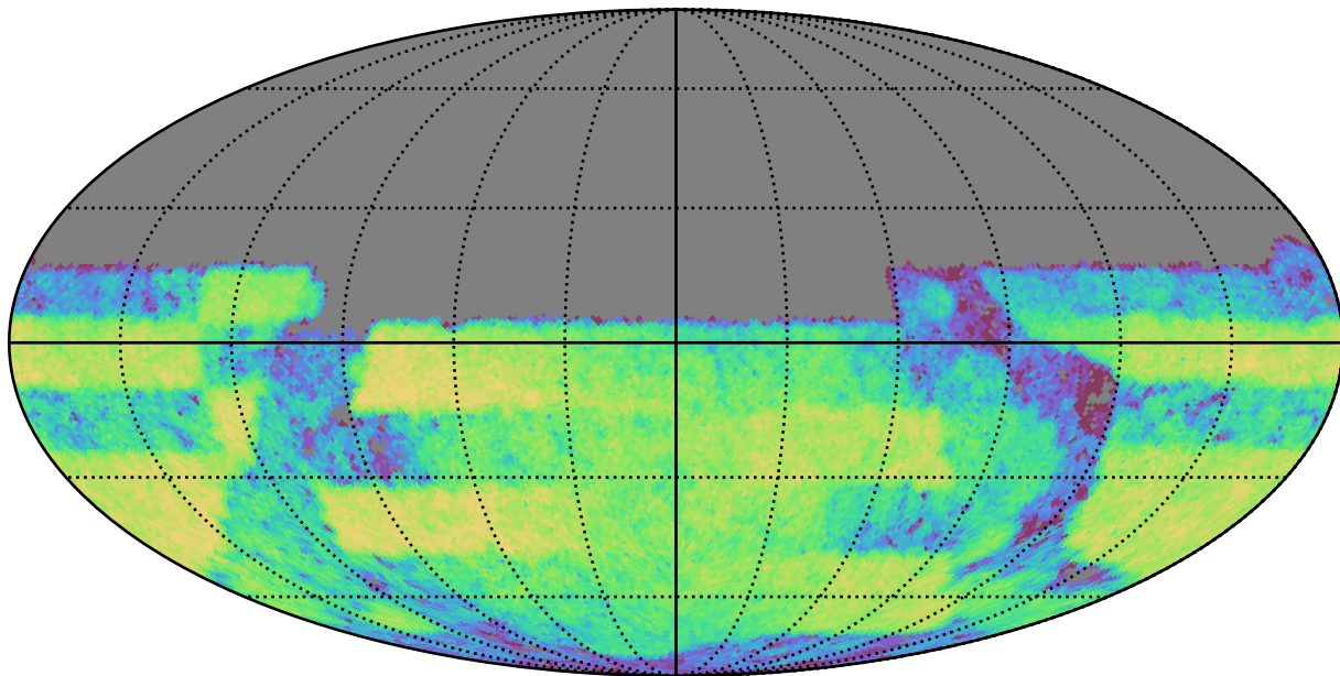
weather_cloudso2v3.4_10yrs Yr 3-4 y band: CoaddM5
