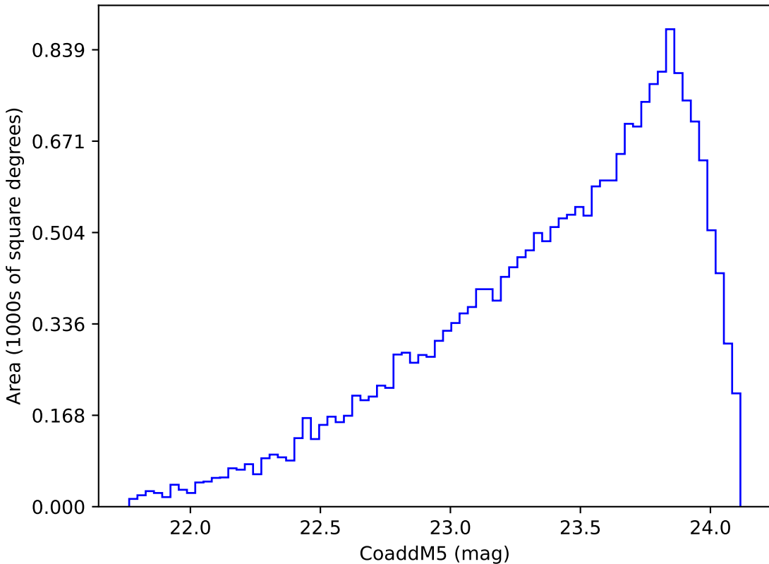
weather_cloudso2v3.4_10yrs Yr 3-4 y band: CoaddM5
