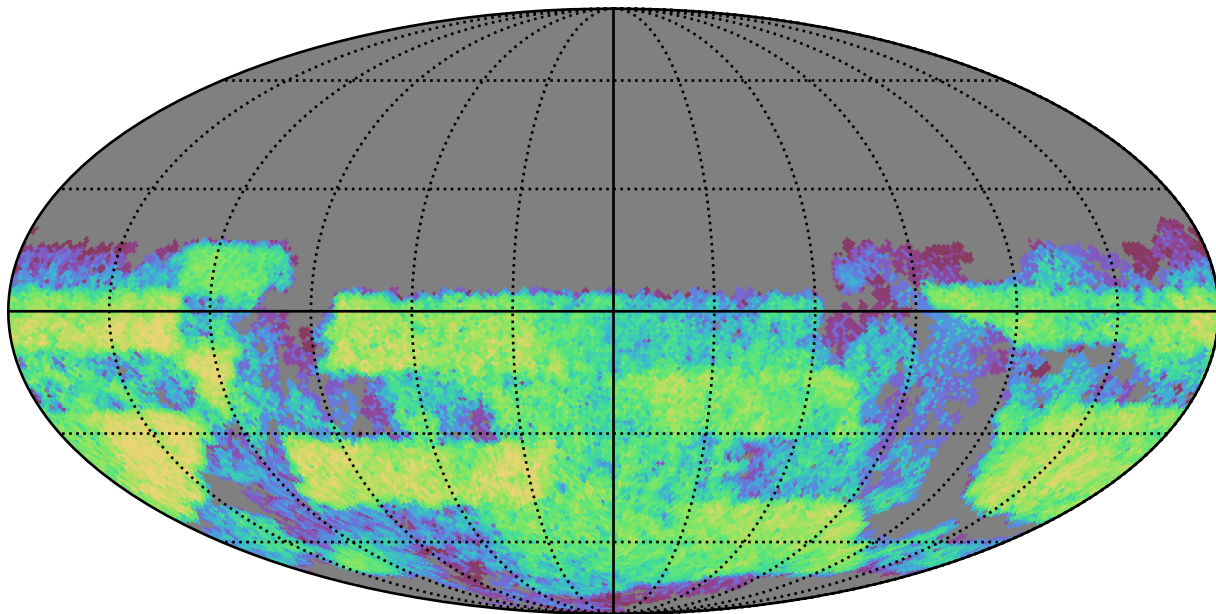
weather_cloudso2v3.4_10yrs Yr 3-4 u band: CoaddM5
