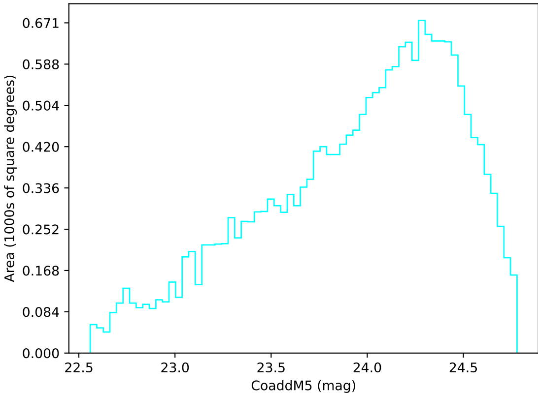
weather_cloudso2v3.4_10yrs Yr 3-4 u band: CoaddM5
