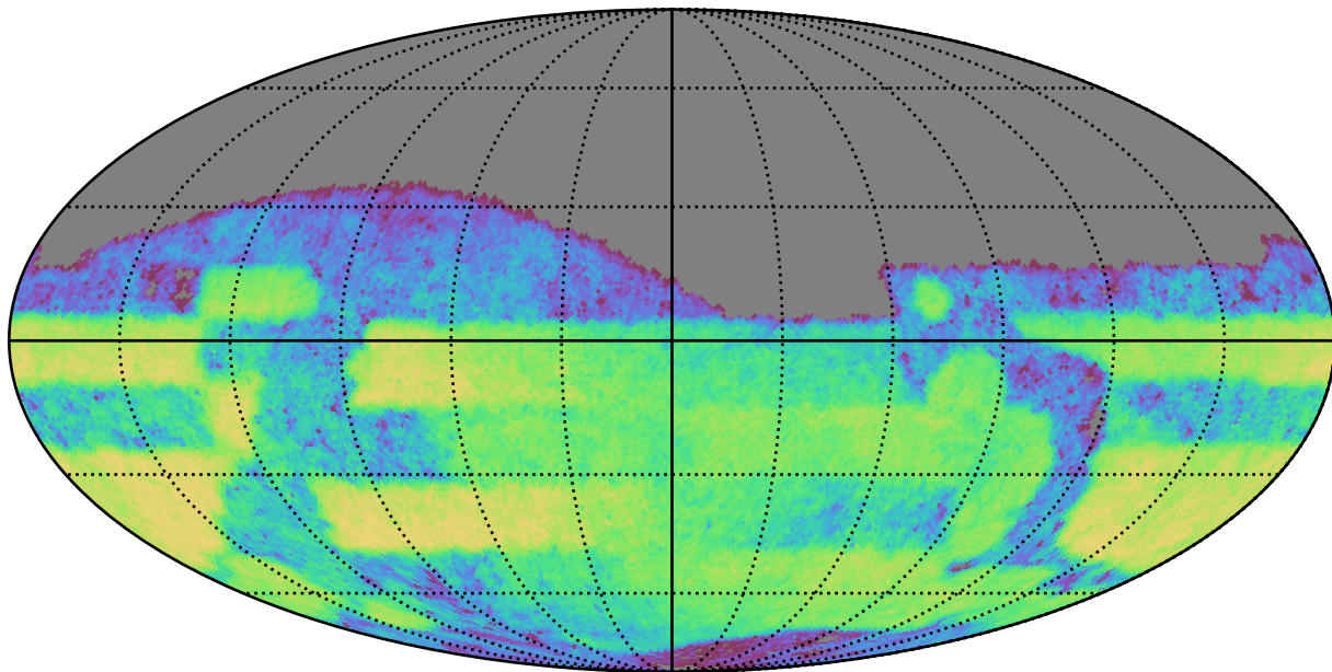
weather_cloudso2v3.4_10yrs Yr 3-4 r band: CoaddM5
