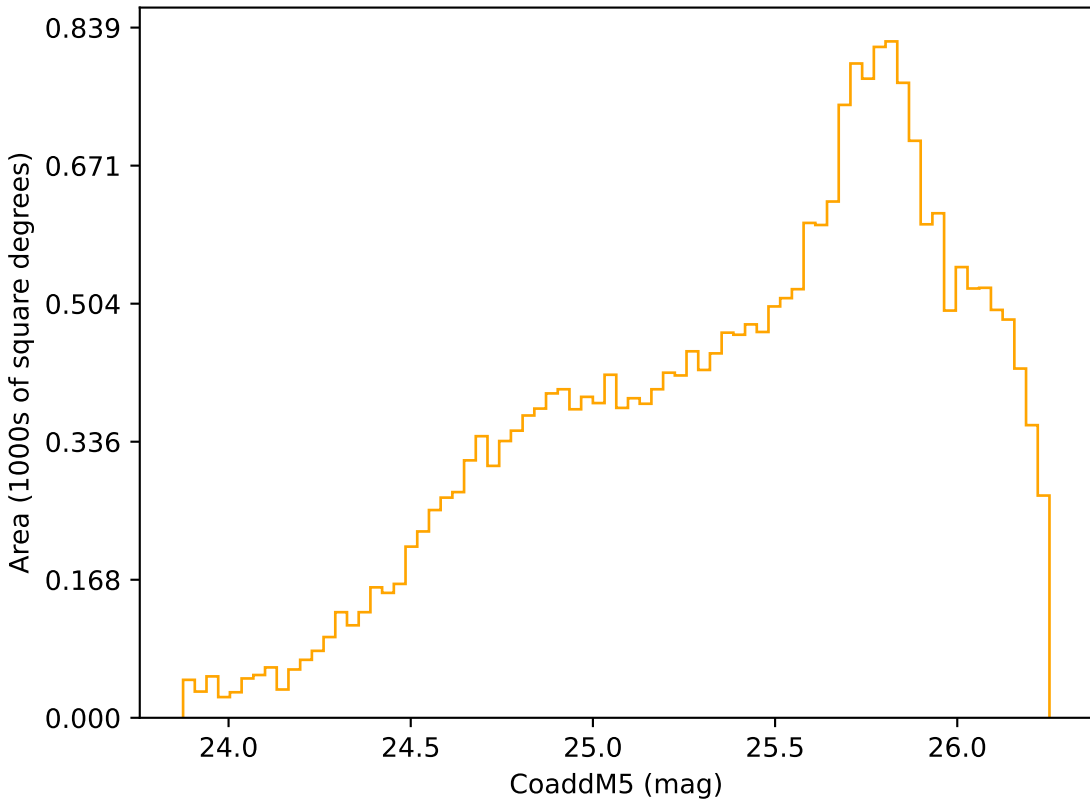
weather_cloudso2v3.4_10yrs Yr 3-4 r band: CoaddM5
