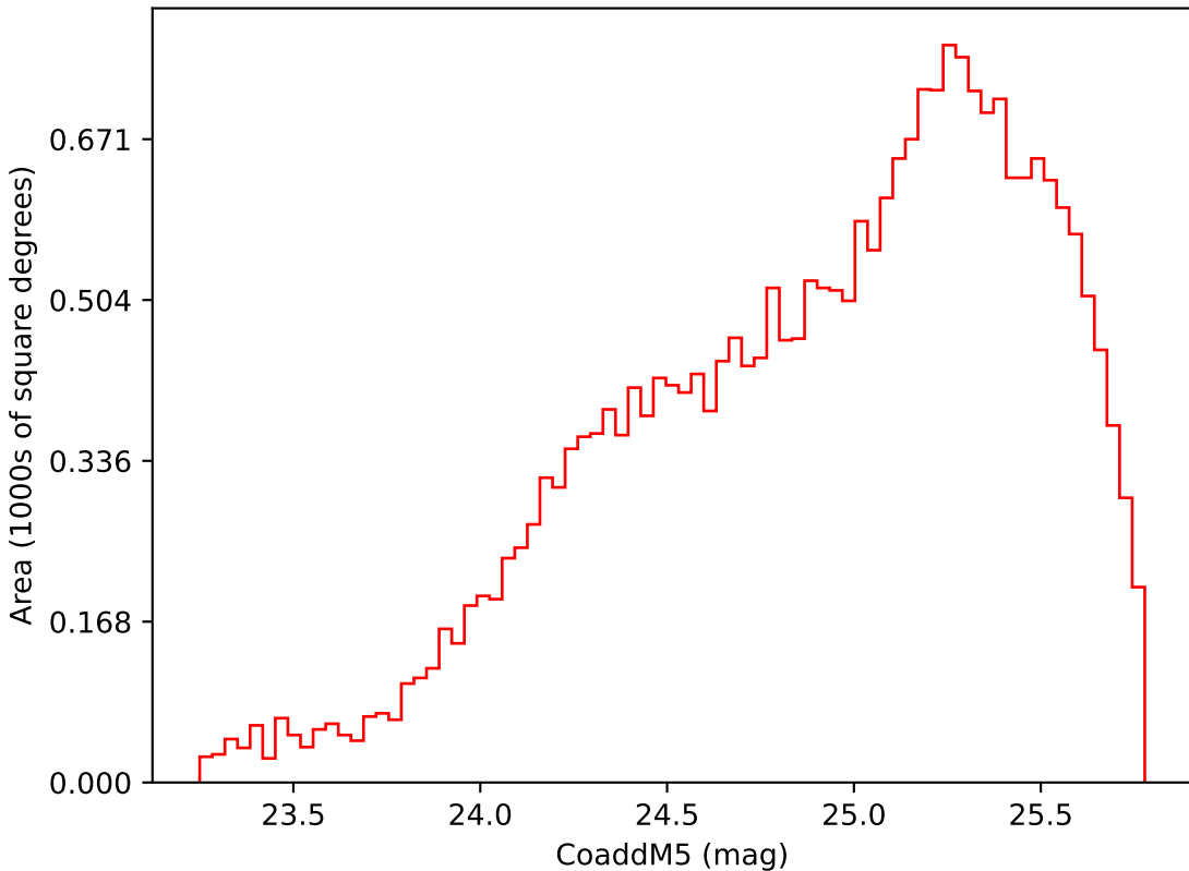
weather_cloudso2v3.4_10yrs Yr 3-4 i band: CoaddM5
