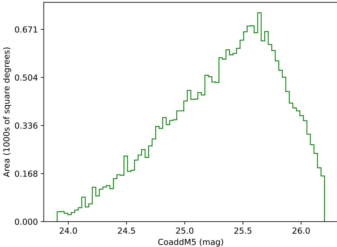
weather_cloudso2v3.4_10yrs Yr 3-4 g band: CoaddM5
