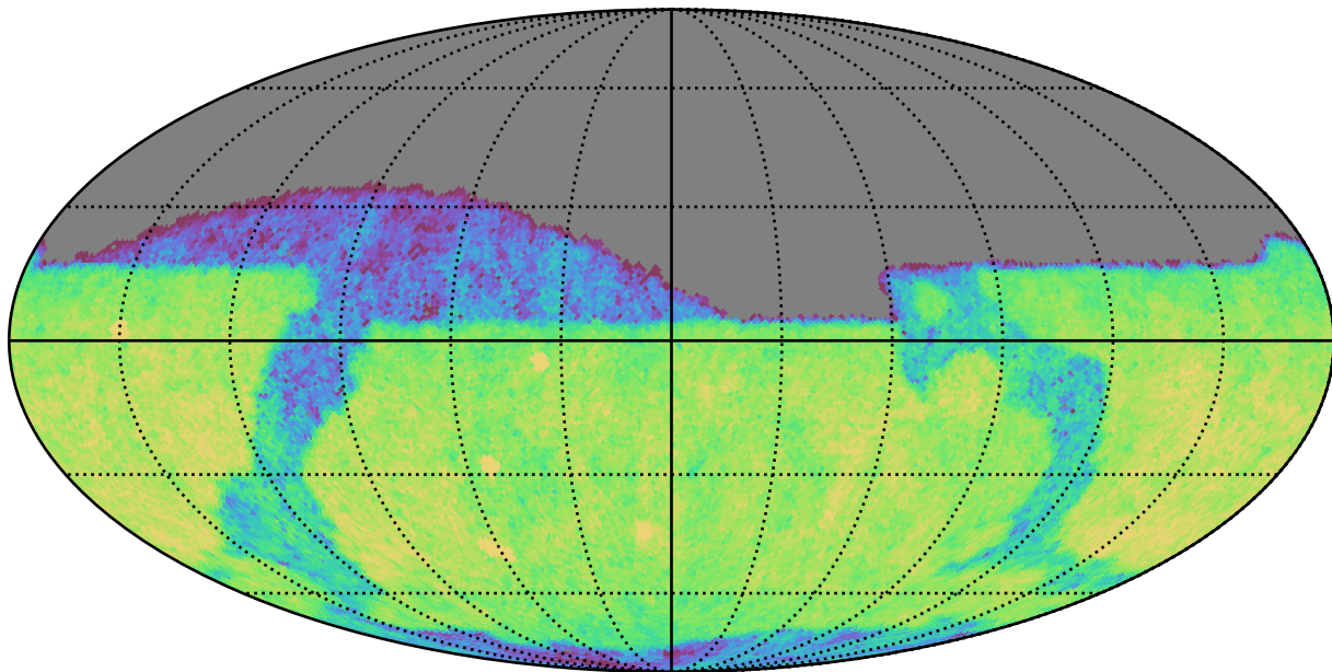
weather_cloudso2v3.4_10yrs Yr 1 z band: CoaddM5
