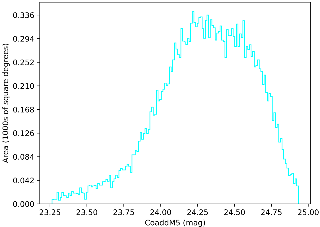
weather_cloudso2v3.4_10yrs Yr 1 u band: CoaddM5
