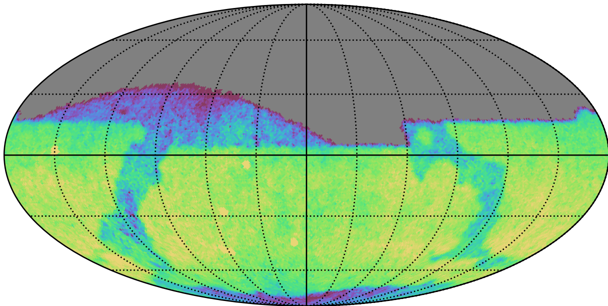
weather_cloudso2v3.4_10yrs Yr 1 r band: CoaddM5
