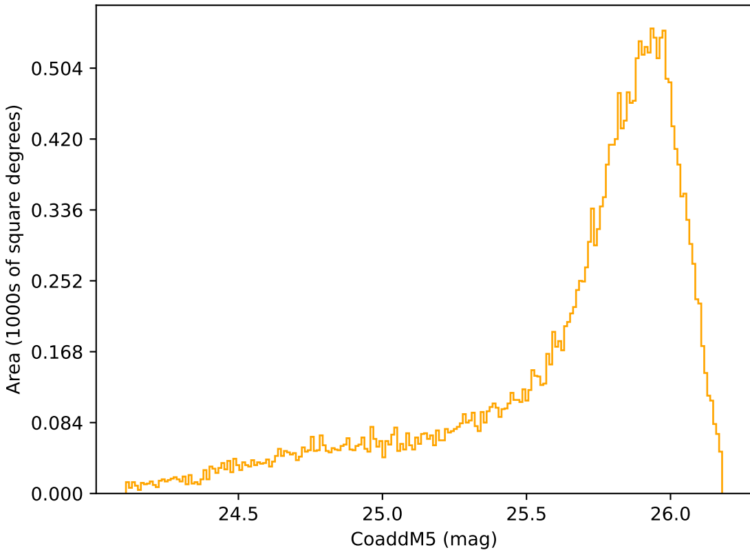
weather_cloudso2v3.4_10yrs Yr 1 r band: CoaddM5
