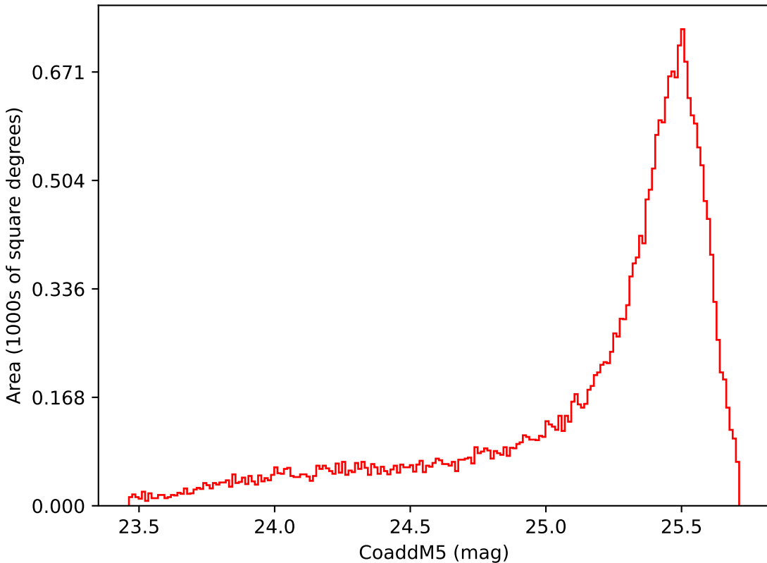
weather_cloudso2v3.4_10yrs Yr 1 i band: CoaddM5
