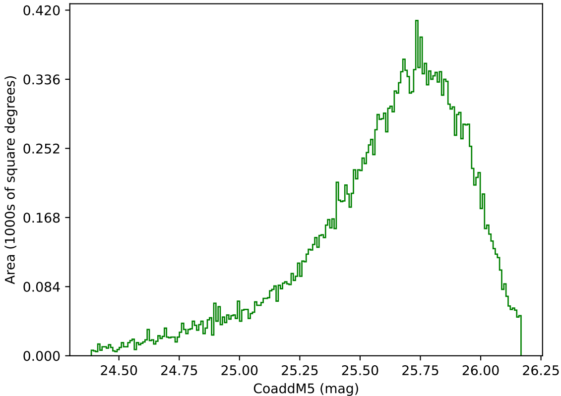
weather_cloudso2v3.4_10yrs Yr 1 g band: CoaddM5
