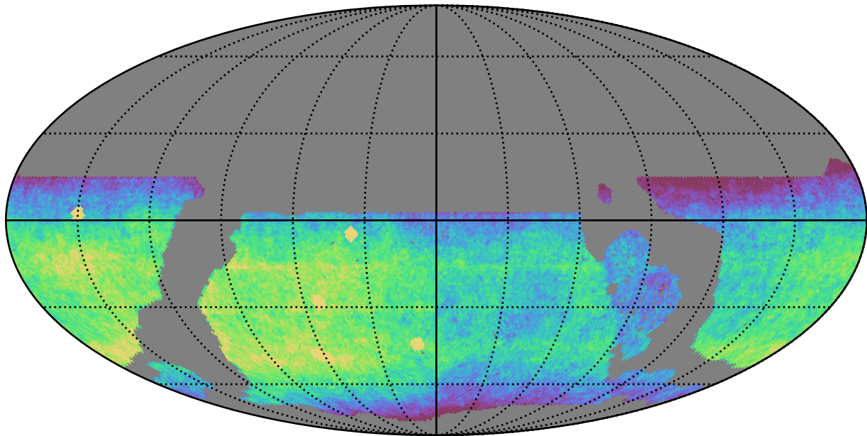
weather_cloudso2v3.4_10yrs WFD z band: CoaddM5
