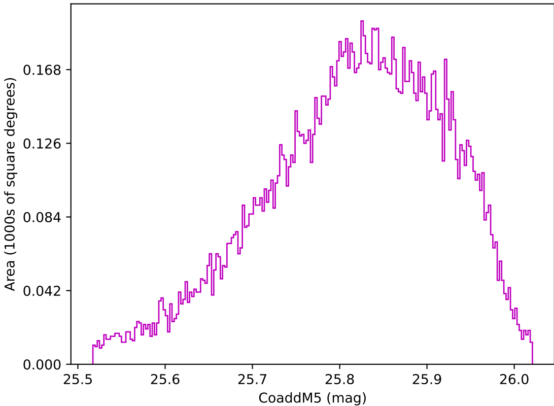
weather_cloudso2v3.4_10yrs WFD z band: CoaddM5
