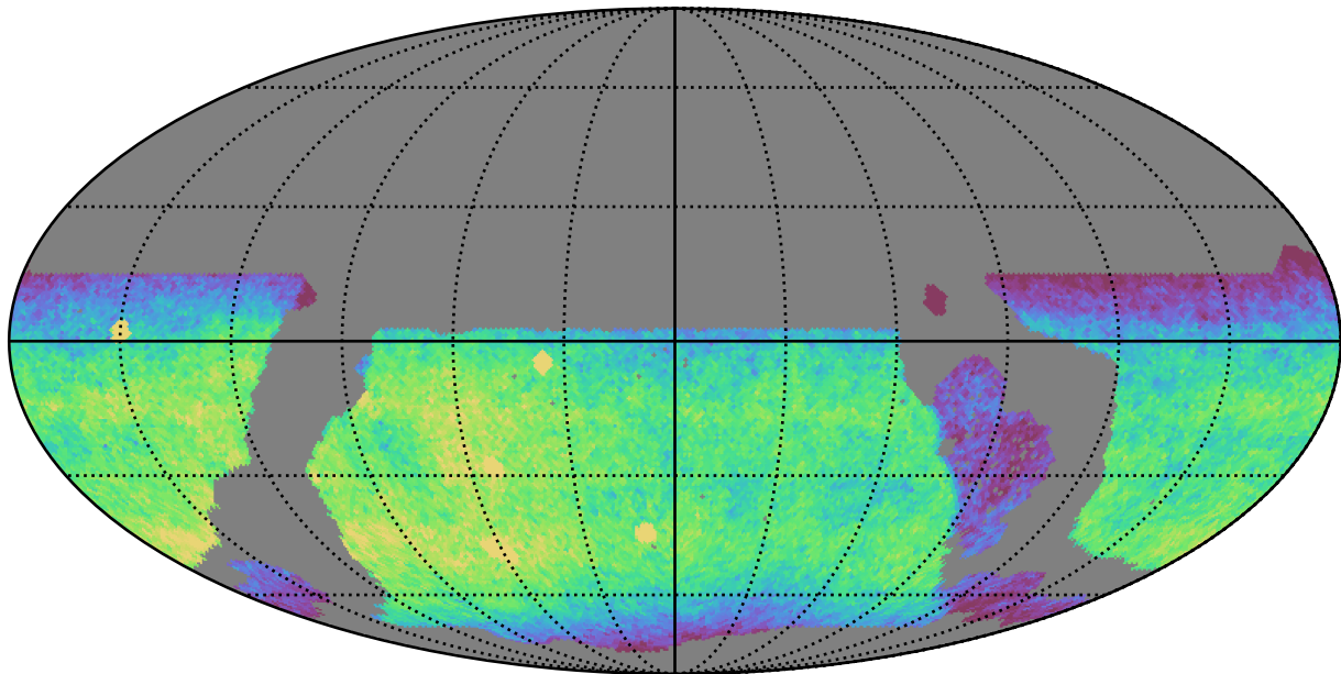
weather_cloudso2v3.4_10yrs WFD y band: CoaddM5
