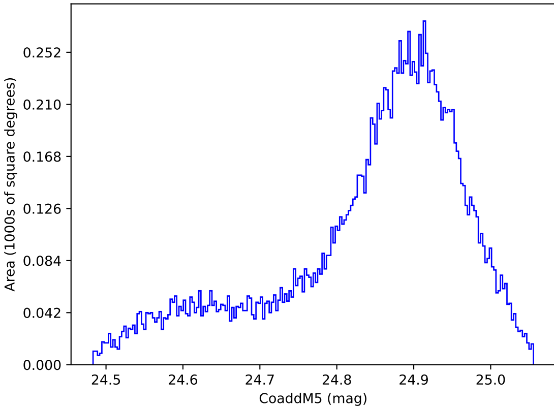
weather_cloudso2v3.4_10yrs WFD y band: CoaddM5
