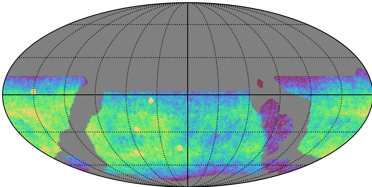
weather_cloudso2v3.4_10yrs WFD u band: CoaddM5
