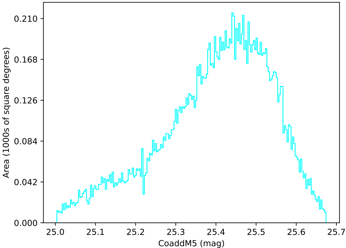
weather_cloudso2v3.4_10yrs WFD u band: CoaddM5
