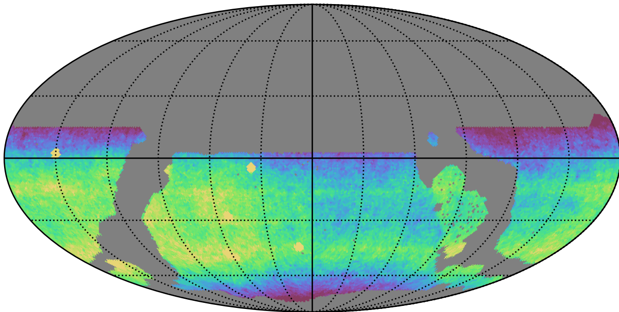
weather_cloudso2v3.4_10yrs WFD r band: CoaddM5
