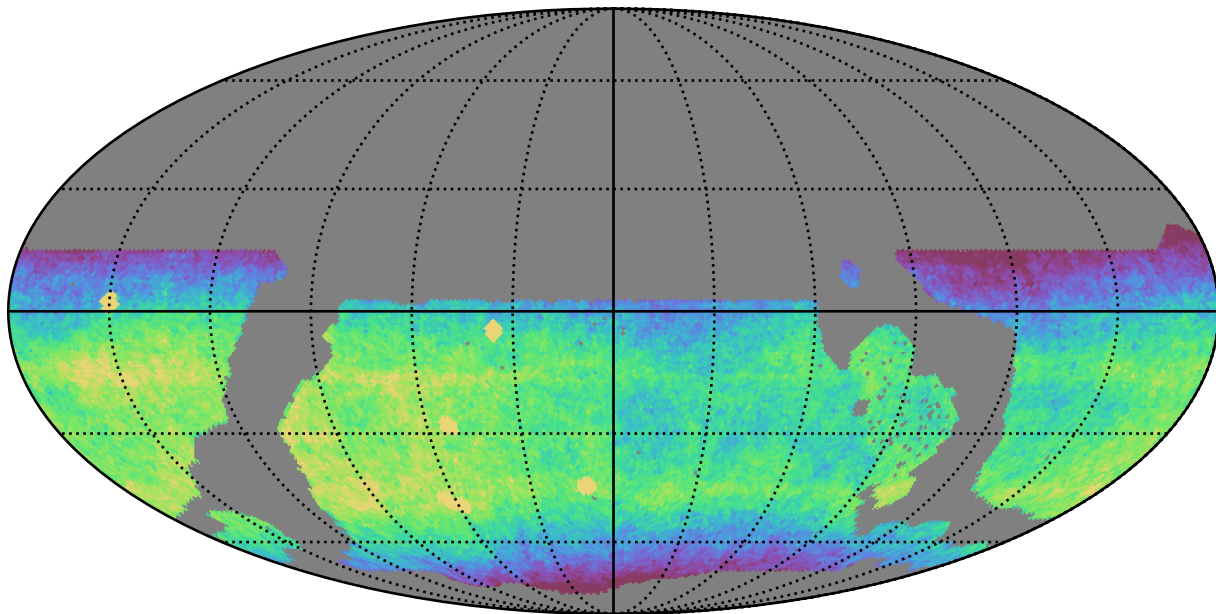
weather_cloudso2v3.4_10yrs WFD i band: CoaddM5
