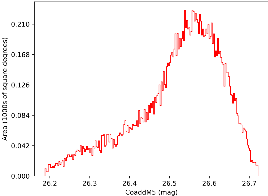
weather_cloudso2v3.4_10yrs WFD i band: CoaddM5
