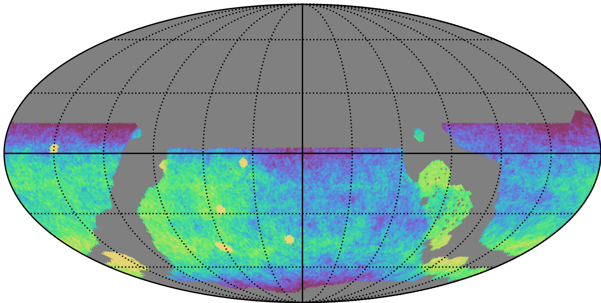
weather_cloudso2v3.4_10yrs WFD g band: CoaddM5
