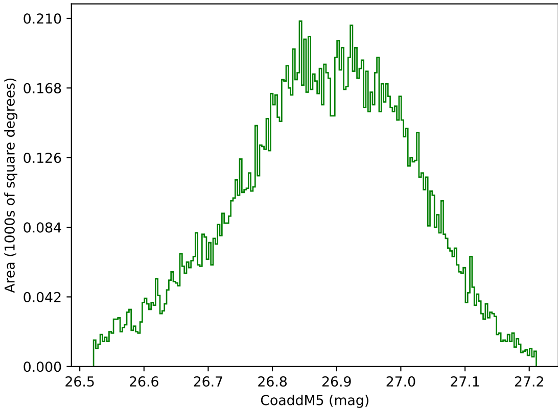
weather_cloudso2v3.4_10yrs WFD g band: CoaddM5
