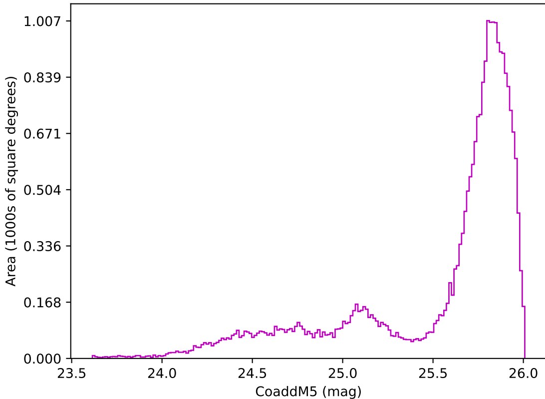
weather_cloudso2v3.4_10yrs All sky z band: CoaddM5
