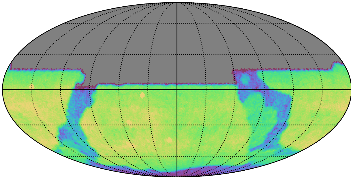
weather_cloudso2v3.4_10yrs All sky u band: CoaddM5
