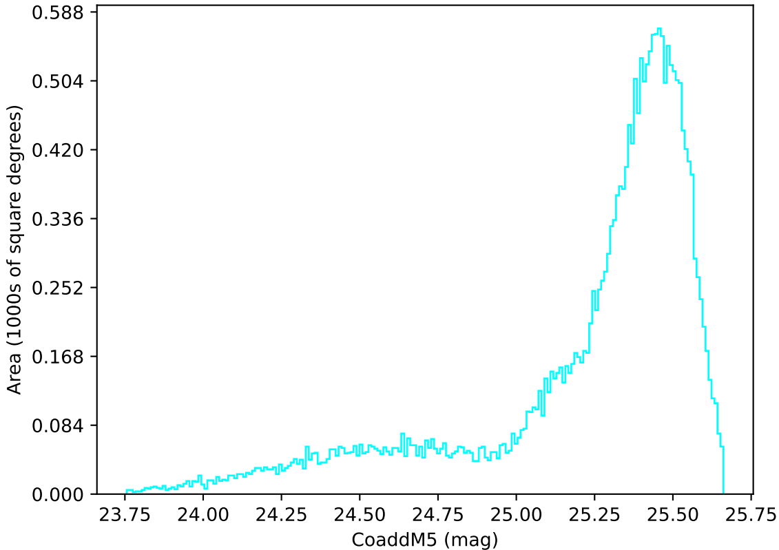
weather_cloudso2v3.4_10yrs All sky u band: CoaddM5
