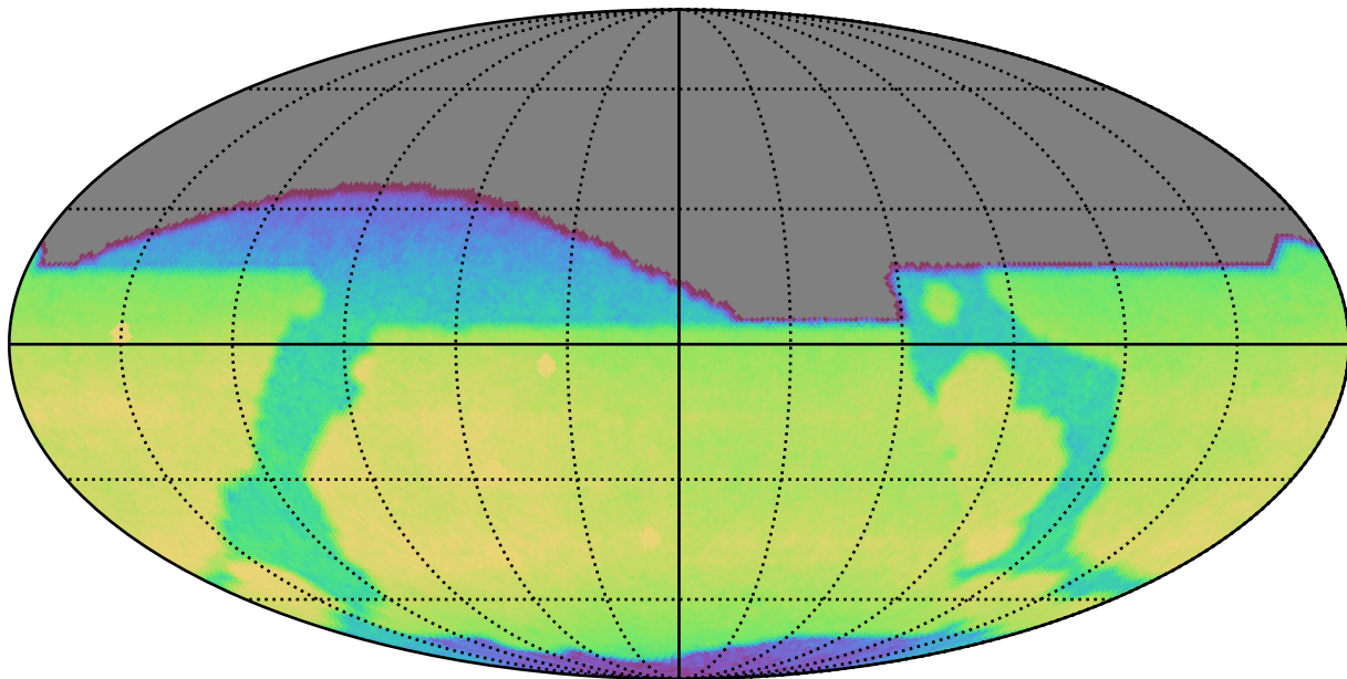
weather_cloudso2v3.4_10yrs All sky r band: CoaddM5
