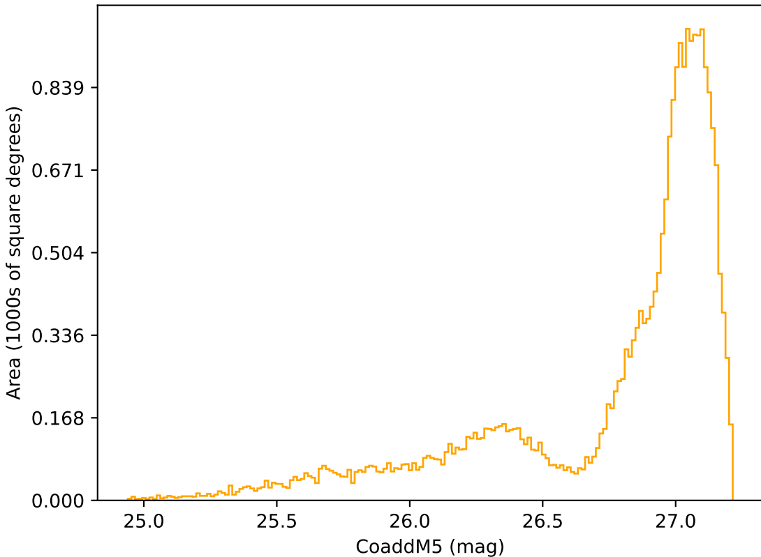
weather_cloudso2v3.4_10yrs All sky r band: CoaddM5
