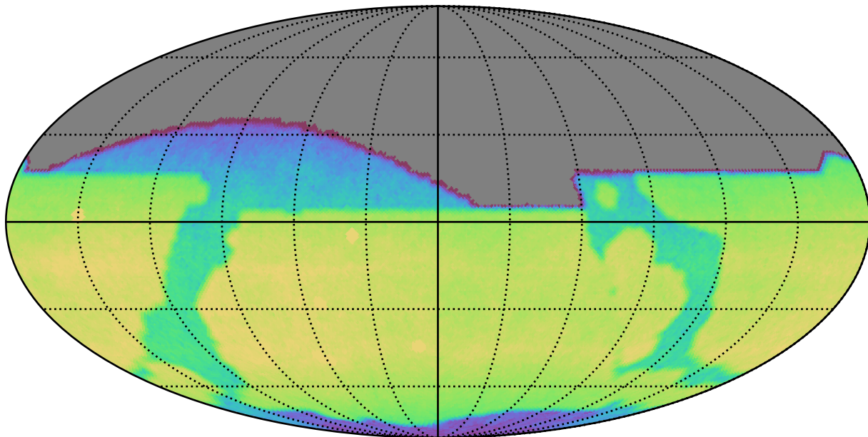
weather_cloudso2v3.4_10yrs All sky i band: CoaddM5
