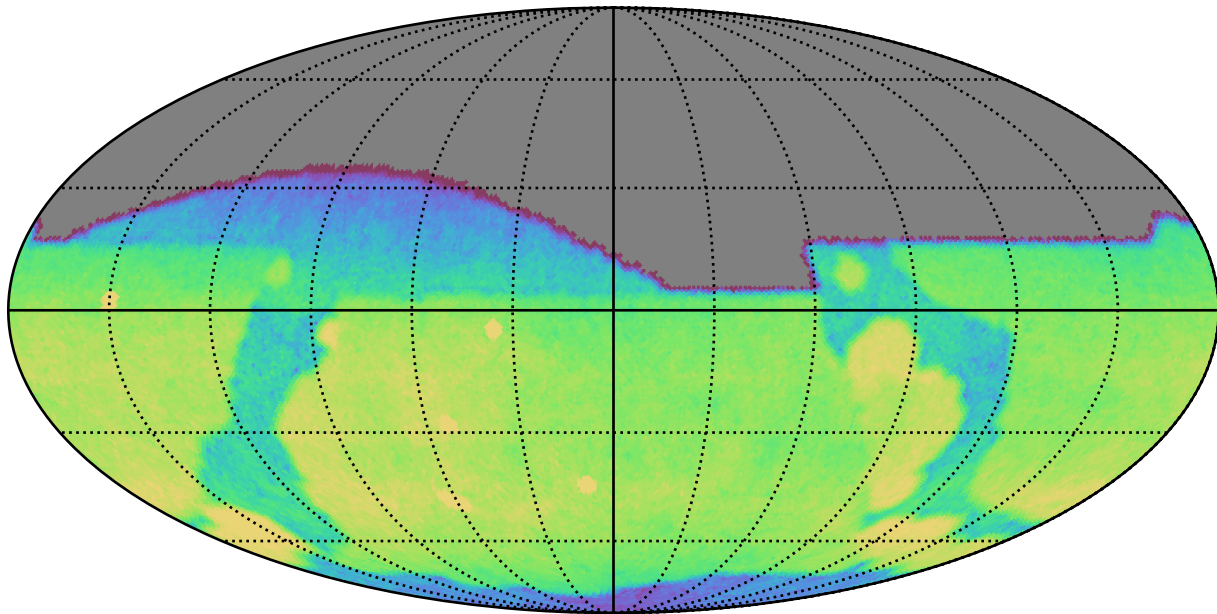
weather_cloudso2v3.4_10yrs All sky g band: CoaddM5
